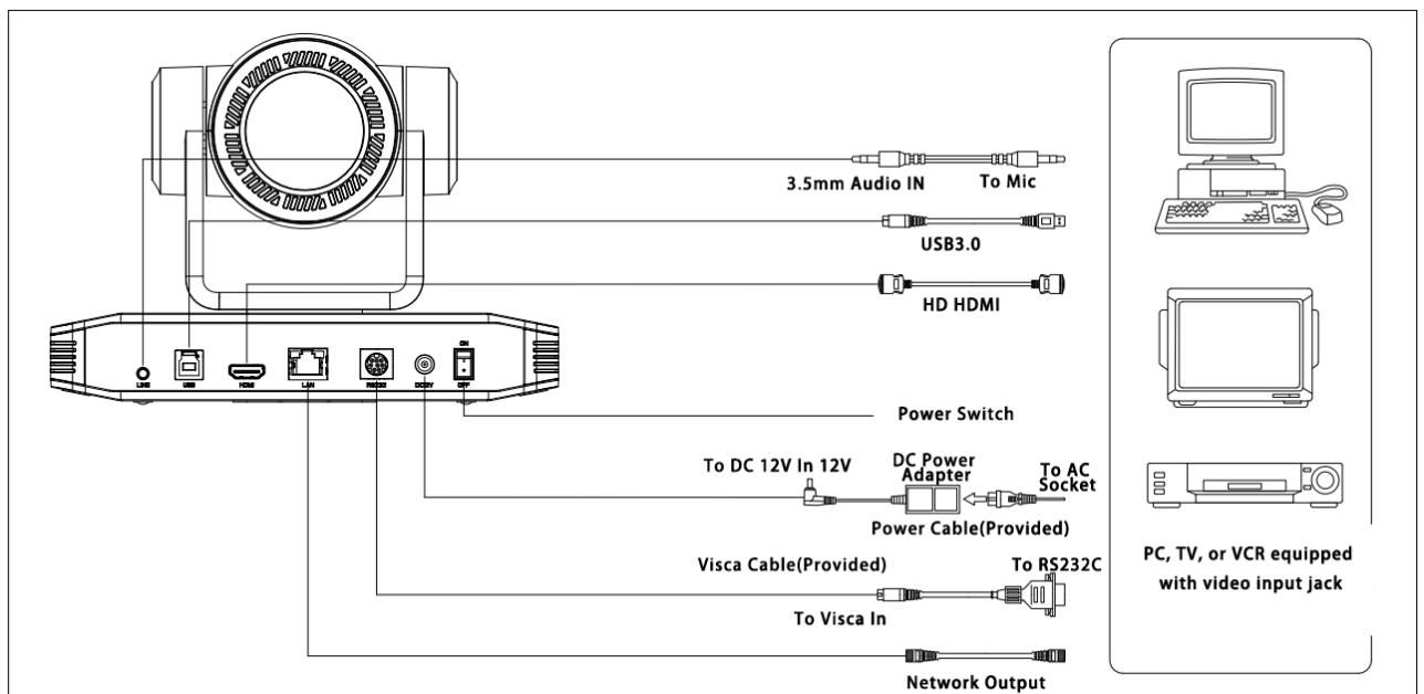
Figure1-5 Interface Diagram
