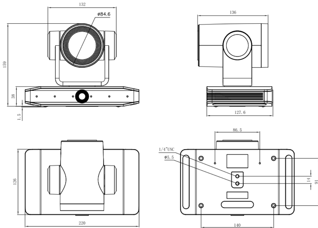
Figure1-4 Product Dimension
