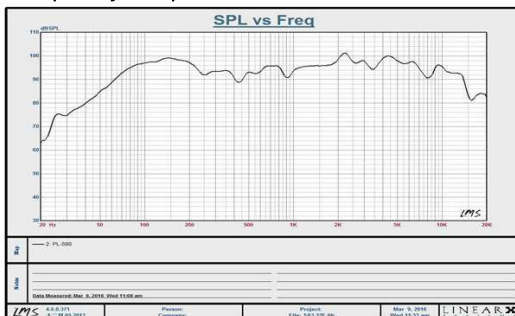
Frequency Response
