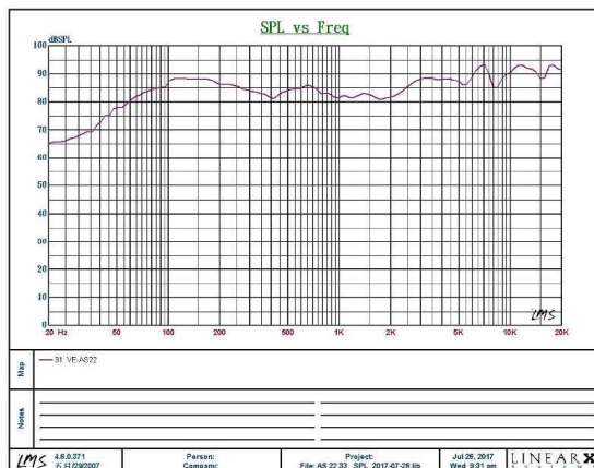
Frequency Response
