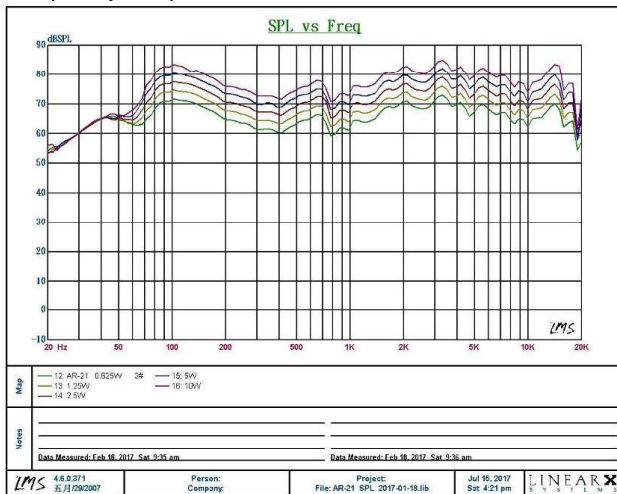
Frequency Response
