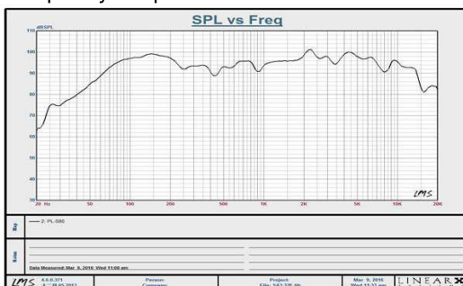
Frequency Response
