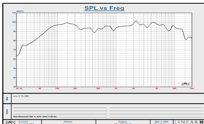
Frequency Response
