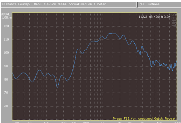
Frequency Response
