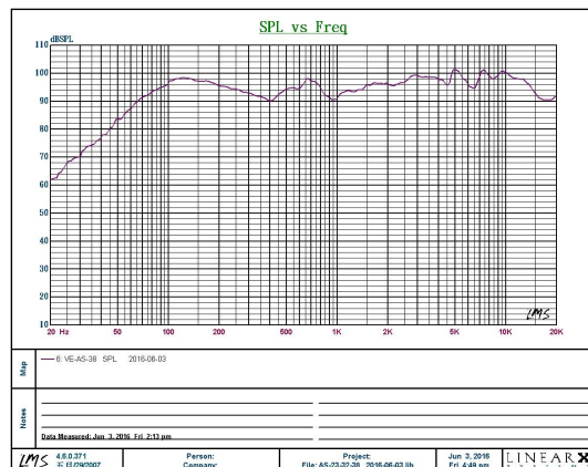
Frequency Response
