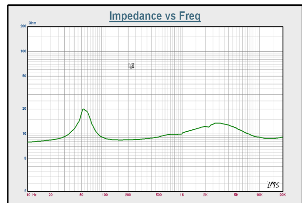
Impedance / Phase
