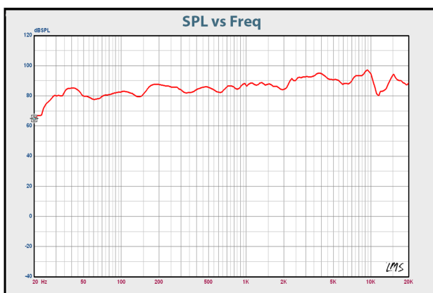
Frequency Response
