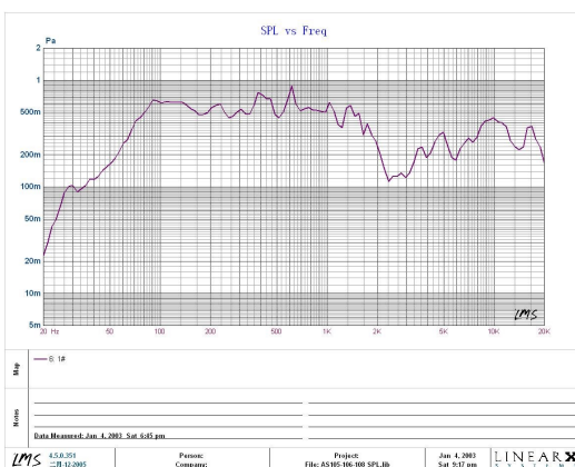
Frequency Response
